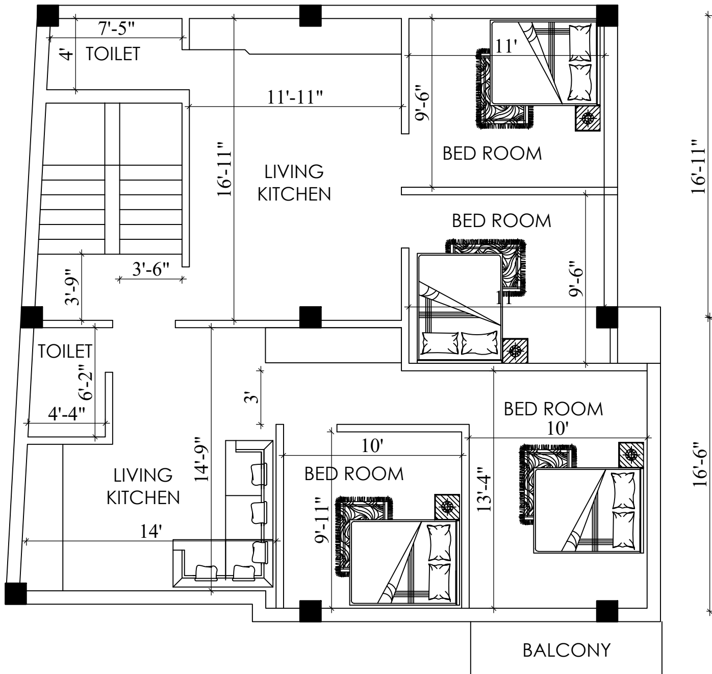
SECOND FLOOR PLAN AREA = 1190 SQ.FT
